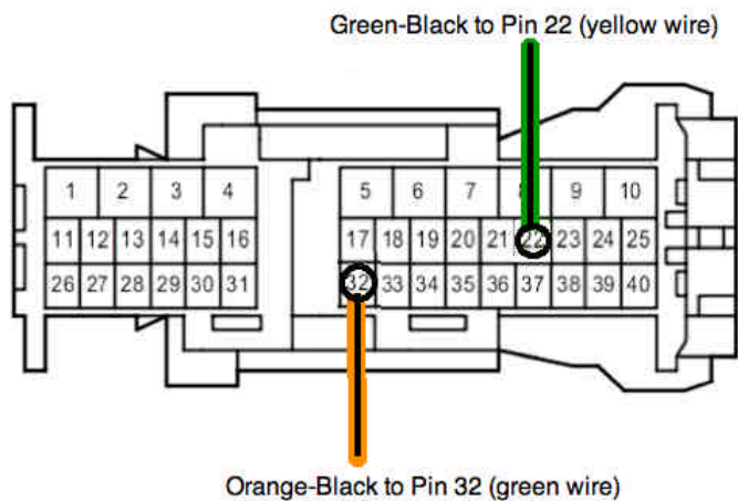
Picture 4: Pin side view
