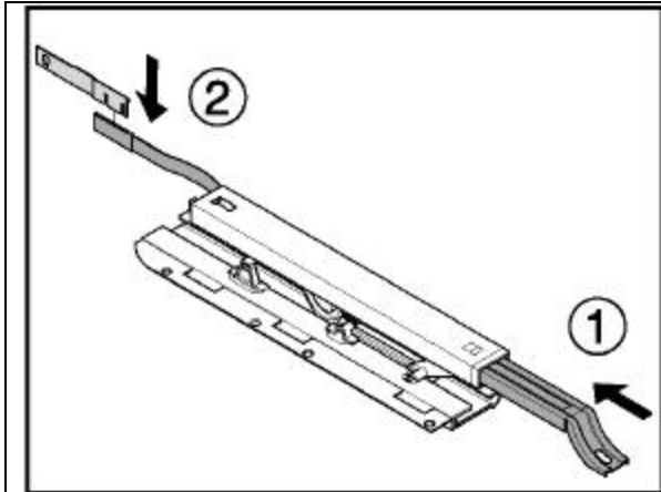
20. Slide the hinge profile in the driving profile and place the fixation plate.
