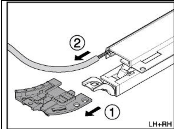
8. Remove the hinge mounting block and driving tubes.
