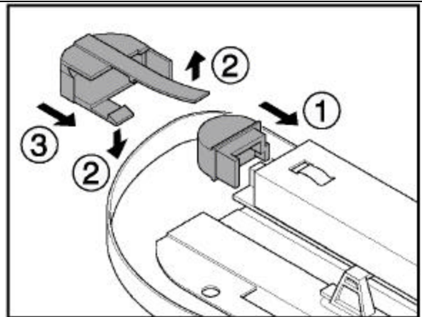
21. Slide the hinge profile in the driving profile and place the fixation plate.
