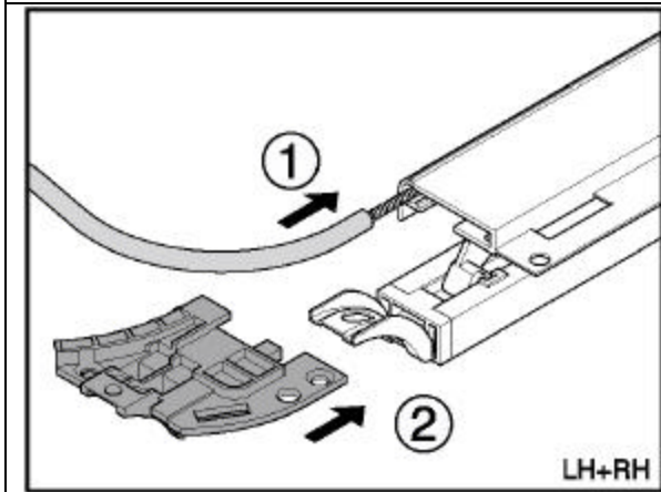
22. Place the cable tubes over the drive cable and make sure that the steel tube is pushed into the mechanism guide. Mount the hinge mounting block.
