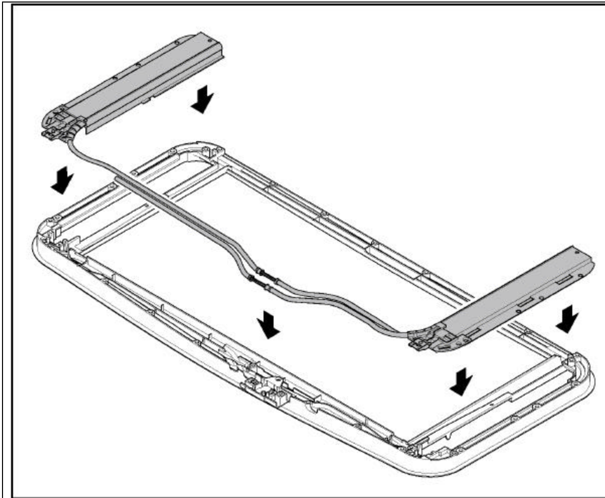
23. The complete mechanism assembly is now ready to be installed on the upper frame.
