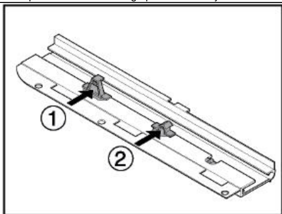
12. Remove the guide insert. Carefully push the guide insert inward on position 1 and 2.
