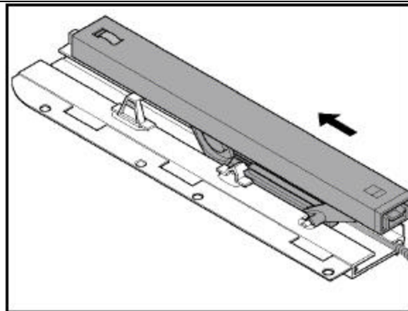
11. Slide the complete mechanism rearwards out of the guide rail.
