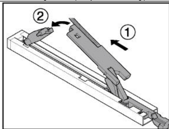
18. Slide the driving slide in the driving profile. Lubricate the driving profile with oil. Connect the driving slide with the front lever.
