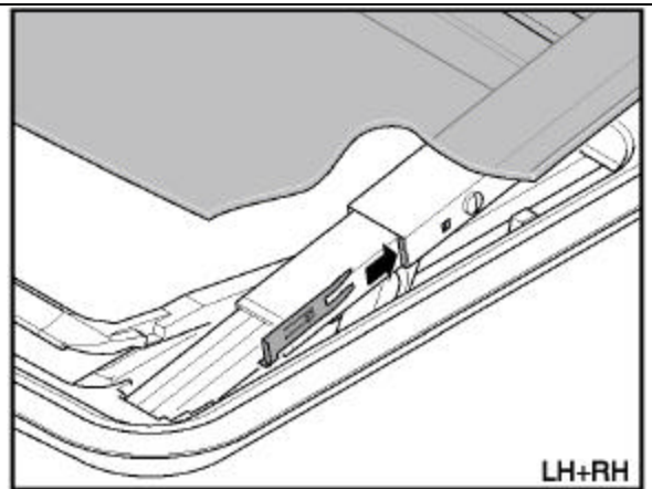
29. Slide the locking part into place to secure the glass panel fixation pin.
