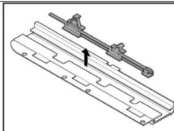
13. Take the guide insert out of the mechanism rail.
