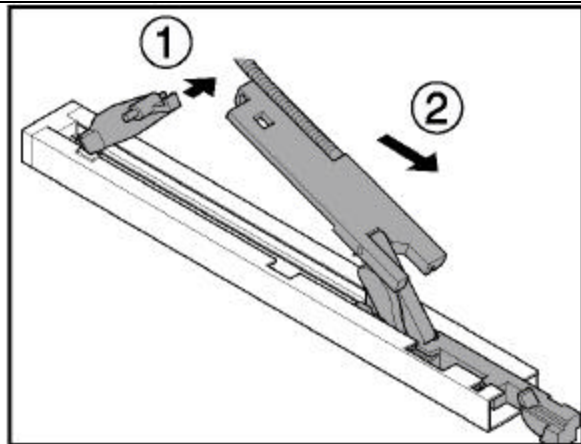
16. Disconnect front lever from the driving slide and slide the driving slide completely out of the driving profile.
