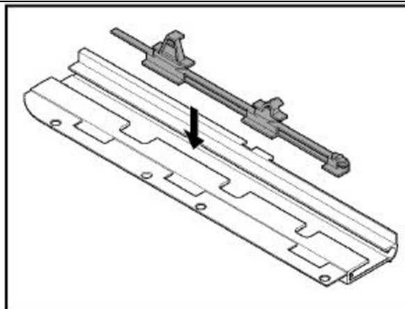
14. Inspect the new guide insert. Place the guide insert in the mechanism rail.
