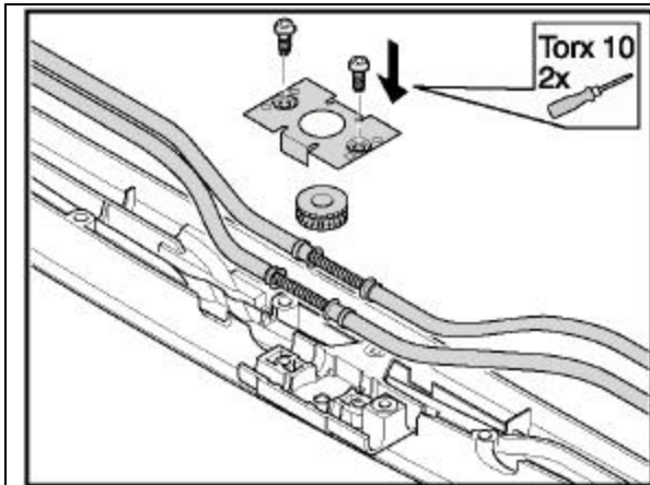
26. Mount the drive cables, gearwheel and gearwheel housing. Align the gearwheel so it is placed in the center of the gearwheel housing.
