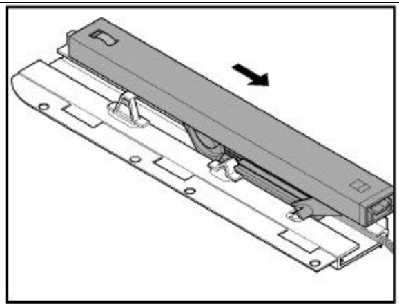
19. Slide the assembled mechanism in the mechanism rail.
