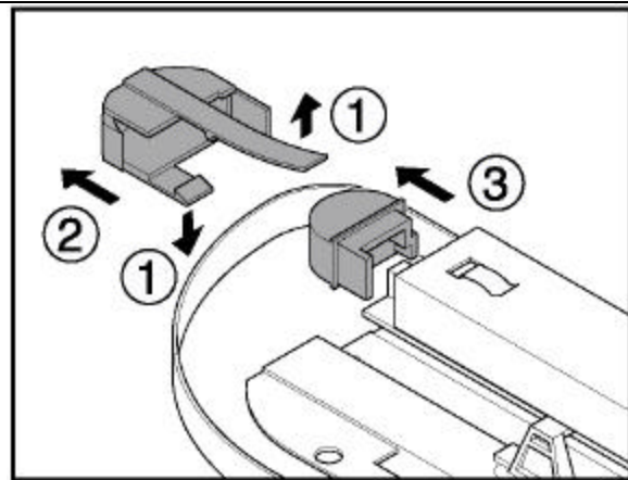
9. Take the hairpin cap from the mechanism by simultaneously lifting the lip upwards and pulling the hairpin cap rearward. Remove the hairpin block.
