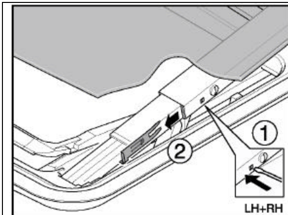
2. Unlock by pushing the screwdriver in the unlocking hole. Slide the locking part forward out of the mechanism. Repeat this at the other side.
