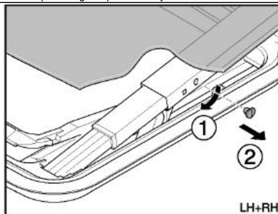
3. Turn the glass panel fixation pin by positioning the flat side parallel with the glass panel and remove it. Repeat for the other side.
