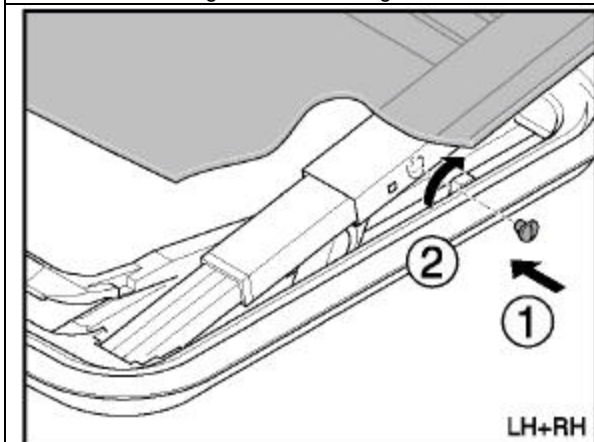
28. Mount the glass panel fixation pin and rotate it 90 degrees to lock it
