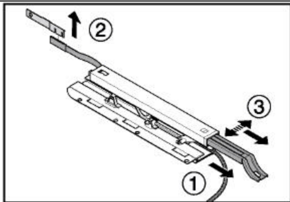
10. Pull the drive cable to place the mechanism in the tilt position. Remove the fixation plate from the hinge profile. Pull the hinge profile out of the mechanism completely. If the hinge profile blocks, simultaneously pull and move the hinge profile side ways.
