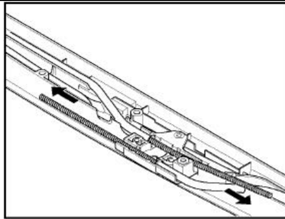
25. Close the mechanism completely by pulling the drive cable till the mechanism is placed in the closed position. Make sure that the hinge belt is not jammed between the mechanism.
