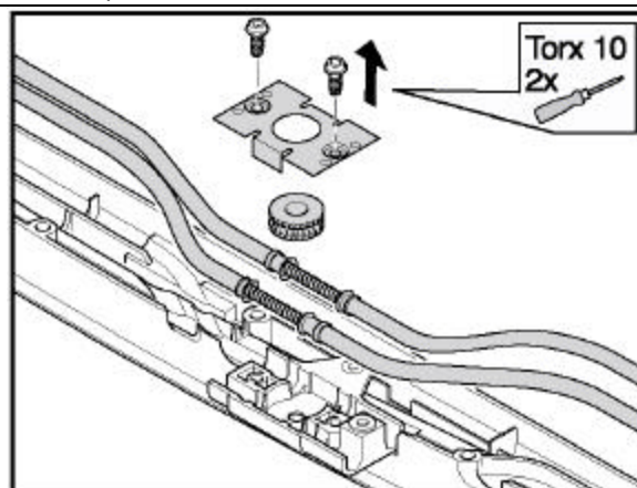
5. Remove gearwheel housing and gearwheel.
